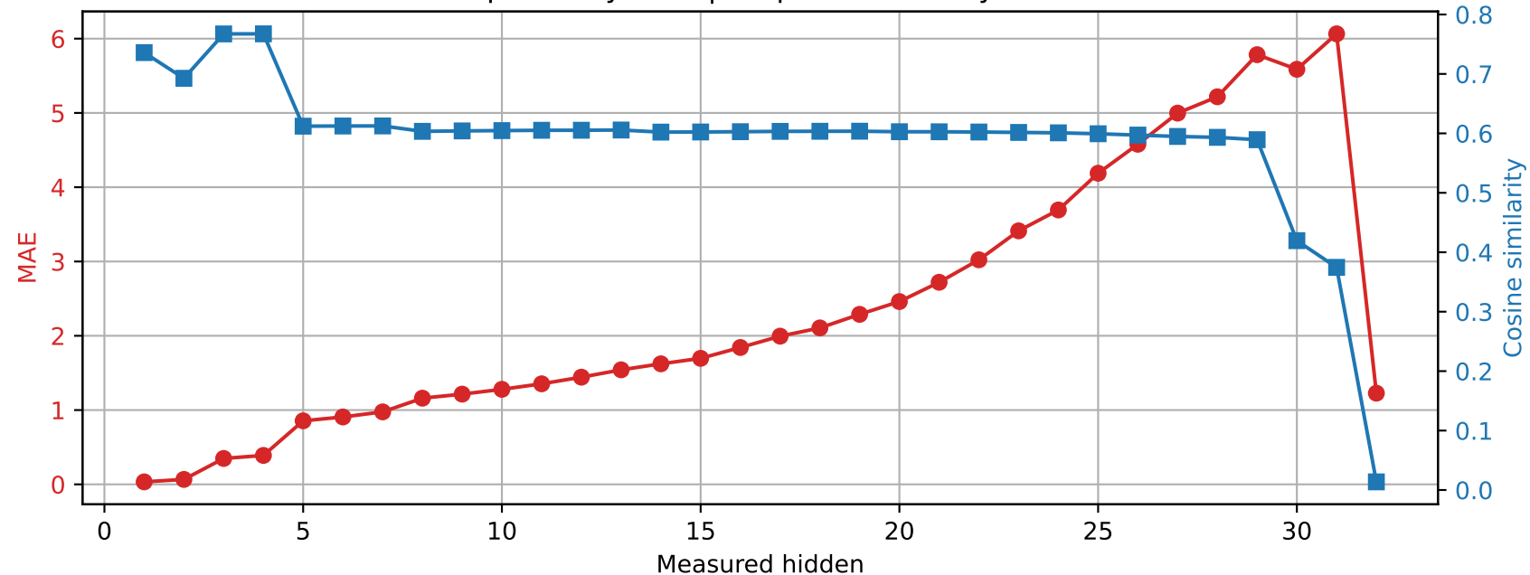
Phi-3-mini-4k-instruct | Prompt 3 Spared layer 17 | Unquantized vs hybrid
