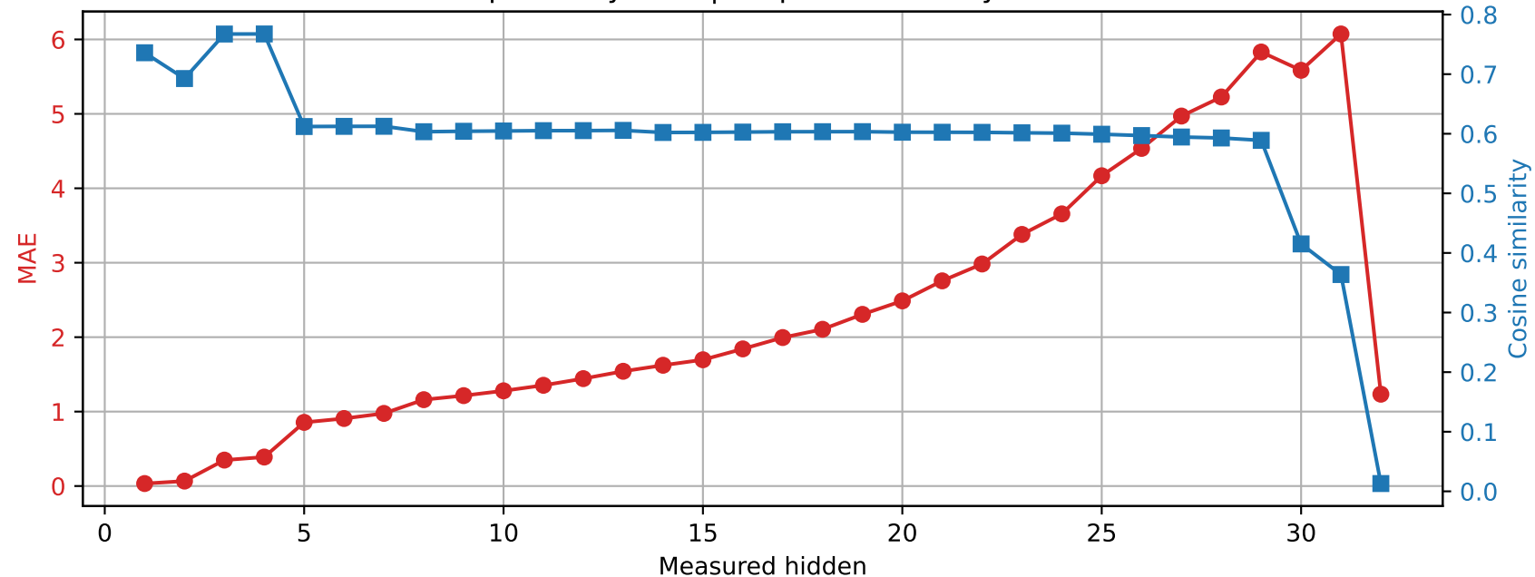
Phi-3-mini-4k-instruct | Prompt 3 Spared layer 21 | Unquantized vs hybrid
