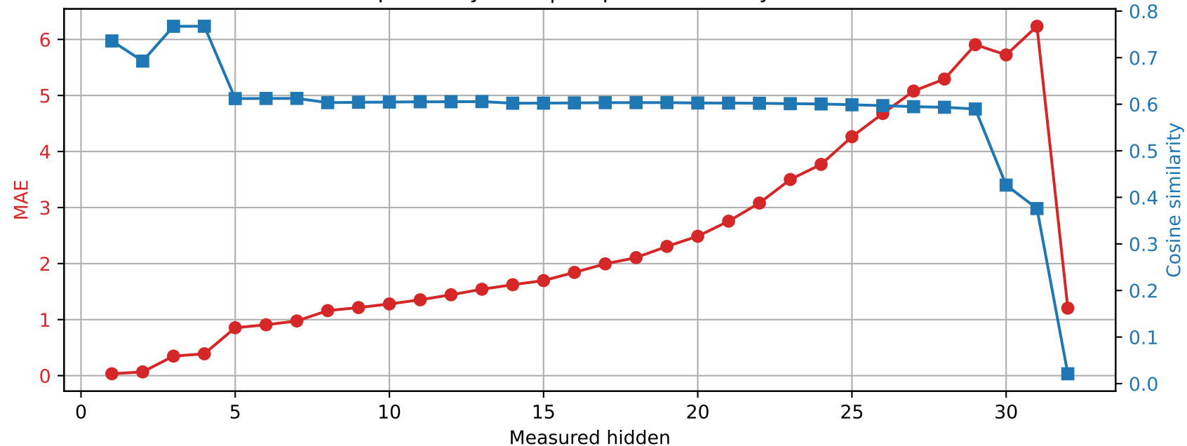
Phi-3-mini-4k-instruct | Prompt 3 Spared layer 25 | Unquantized vs hybrid
