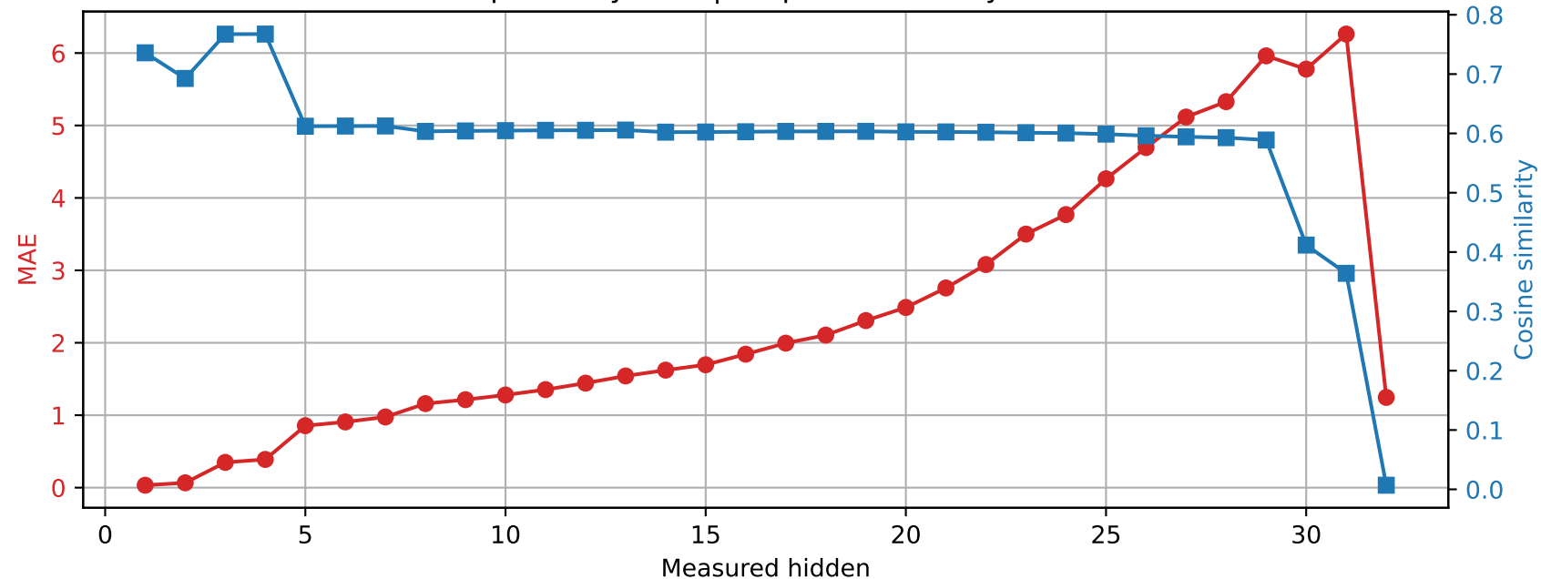
Phi-3-mini-4k-instruct | Prompt 3 Spared layer 26 | Unquantized vs hybrid
