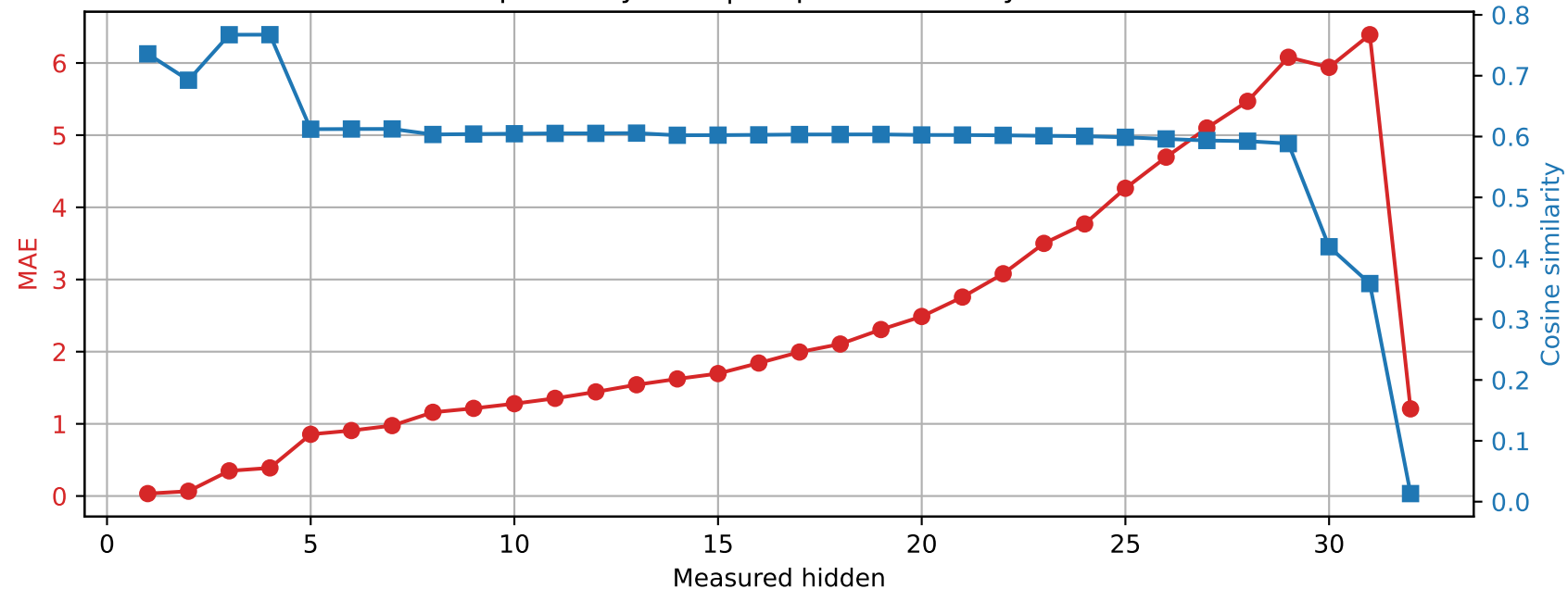
Phi-3-mini-4k-instruct | Prompt 3 Spared layer 27 | Unquantized vs hybrid
