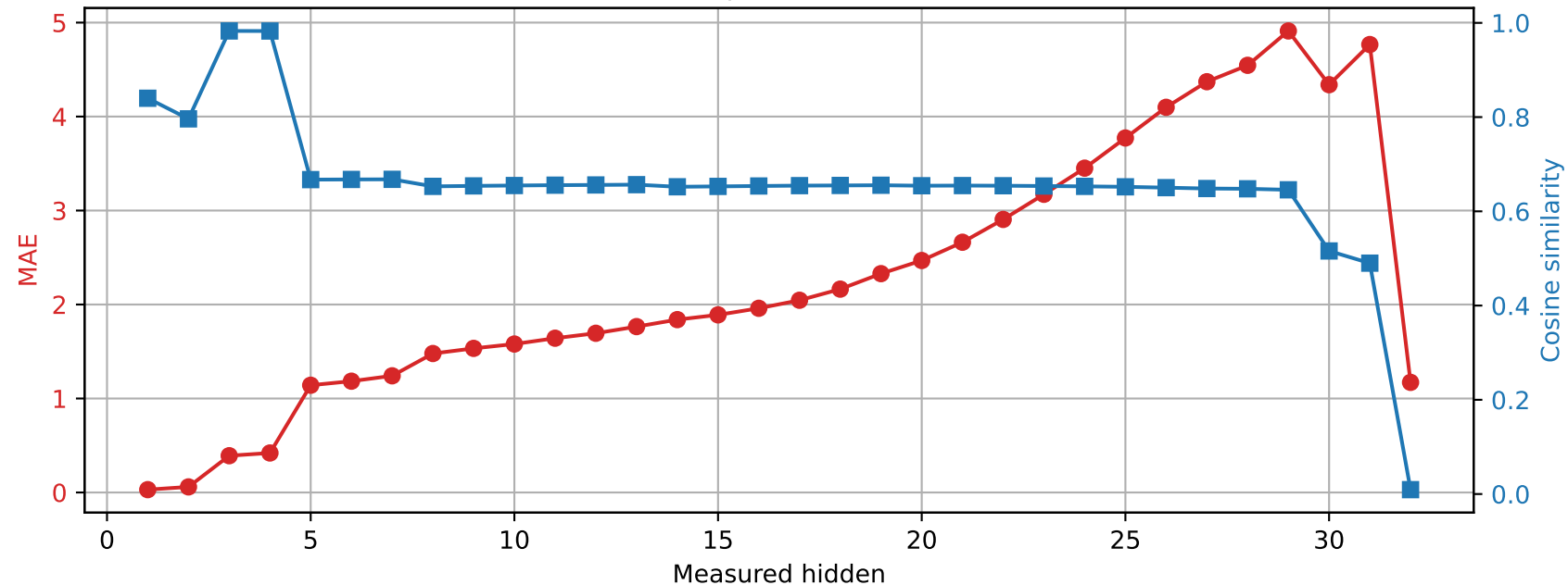
Phi-3-mini-4k-instruct | Prompt 4 Spared layer 15 | Unquantized vs hybrid
