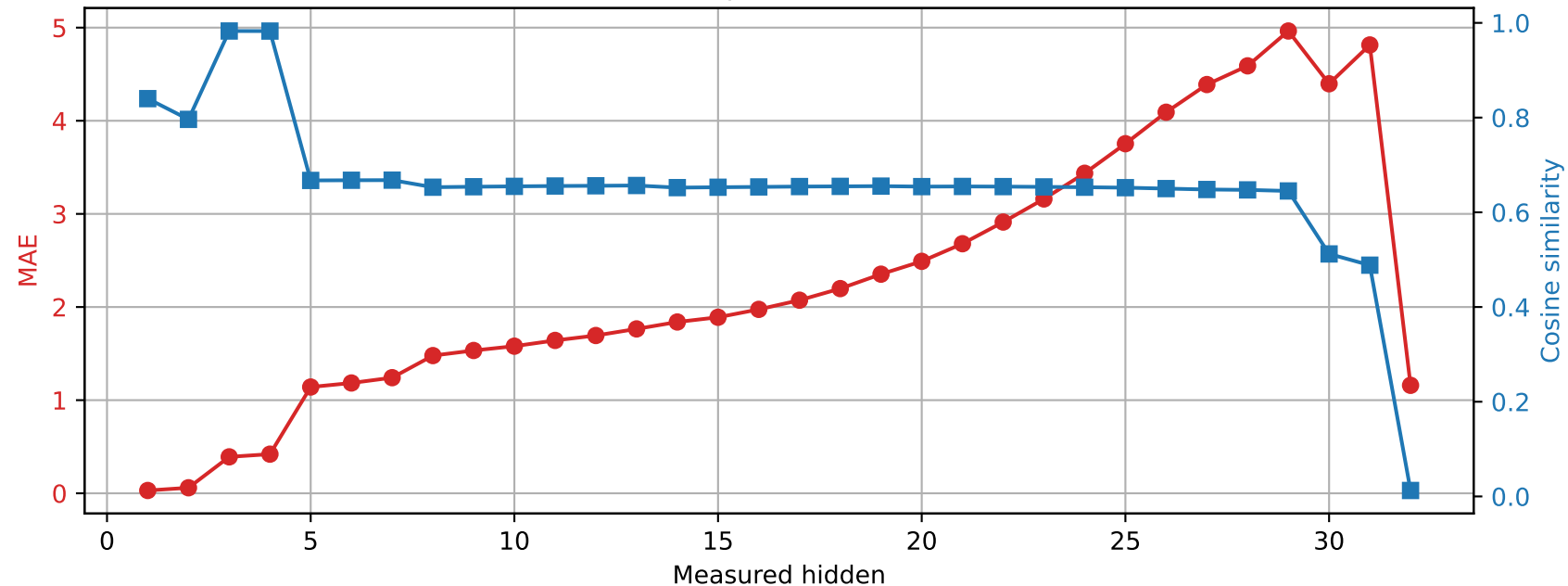
Phi-3-mini-4k-instruct | Prompt 4 Spared layer 18 | Unquantized vs hybrid
