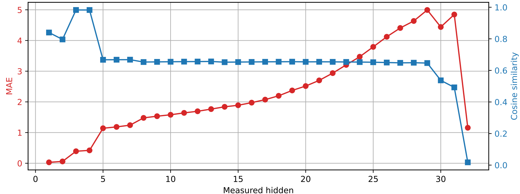
Phi-3-mini-4k-instruct | Prompt 4 Spared layer 27 | Unquantized vs hybrid
