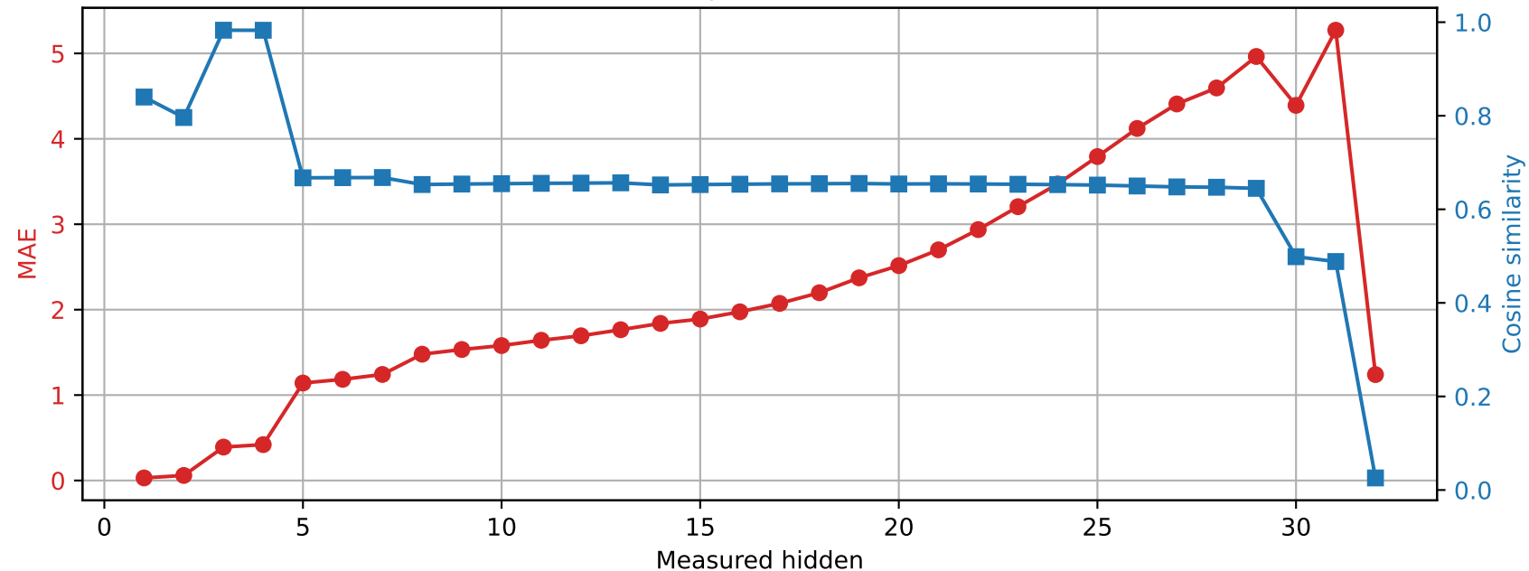
Phi-3-mini-4k-instruct | Prompt 4 Spared layer 30 | Unquantized vs hybrid
