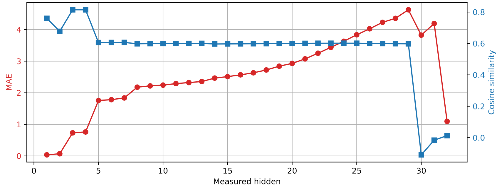
Phi-3-mini-4k-instruct | Prompt 0 Spared layer 4 | Unquantized vs hybrid
