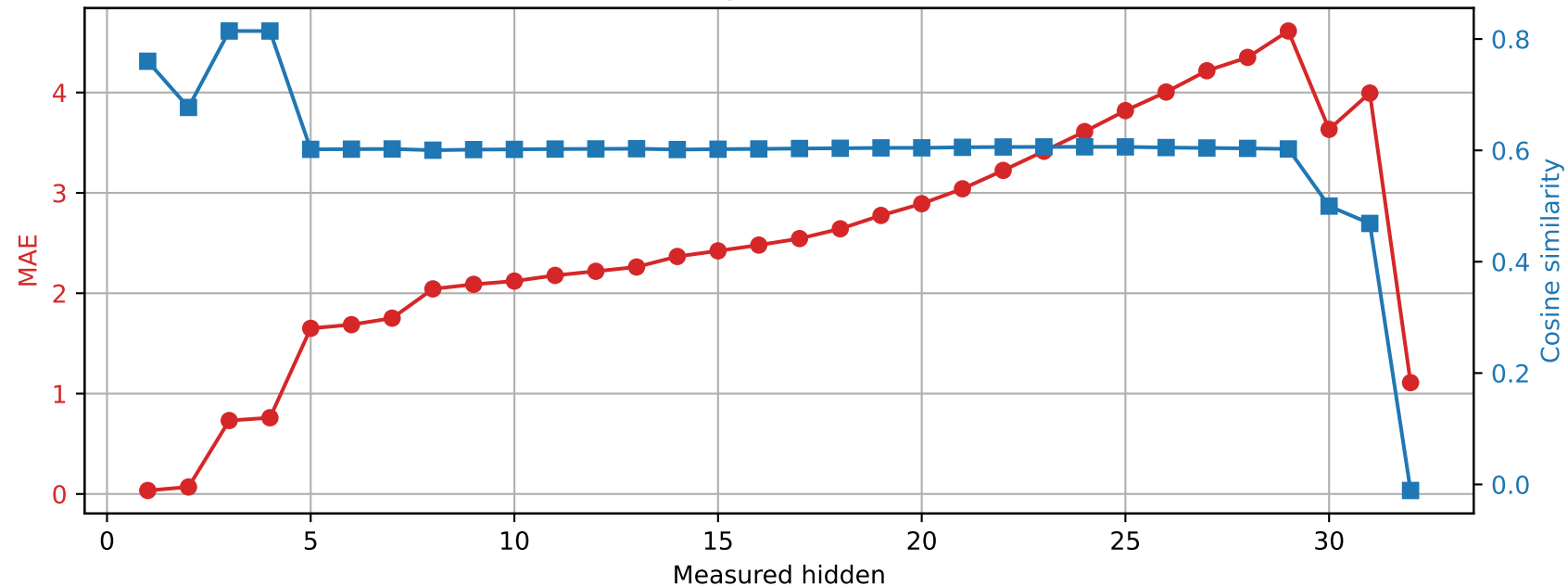
Phi-3-mini-4k-instruct | Prompt 0 Spared layer 14 | Unquantized vs hybrid
