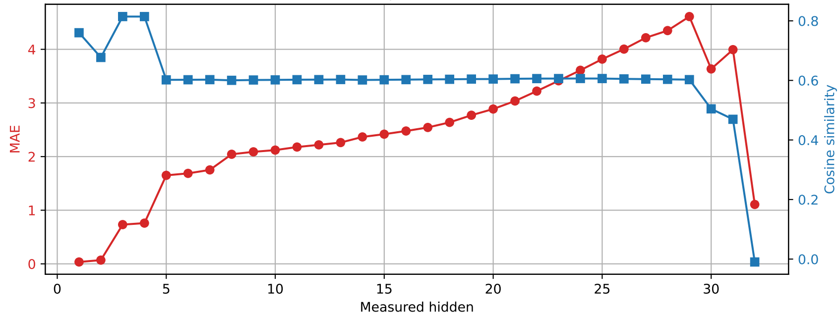
Phi-3-mini-4k-instruct | Prompt 0 Spared layer 15 | Unquantized vs hybrid
