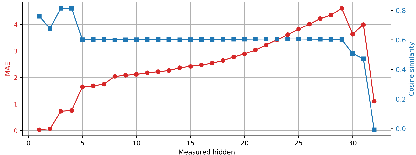
Phi-3-mini-4k-instruct | Prompt 0 Spared layer 22 | Unquantized vs hybrid
