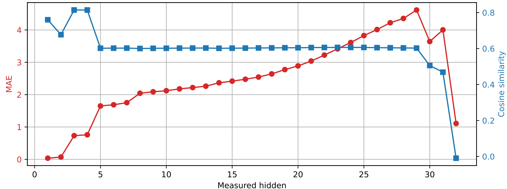
Phi-3-mini-4k-instruct | Prompt 0 Spared layer 24 | Unquantized vs hybrid
