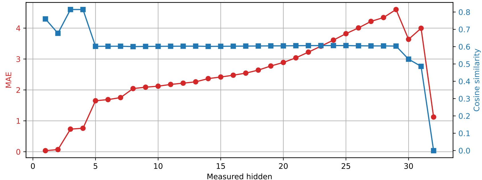
Phi-3-mini-4k-instruct | Prompt 0 Spared layer 27 | Unquantized vs hybrid
