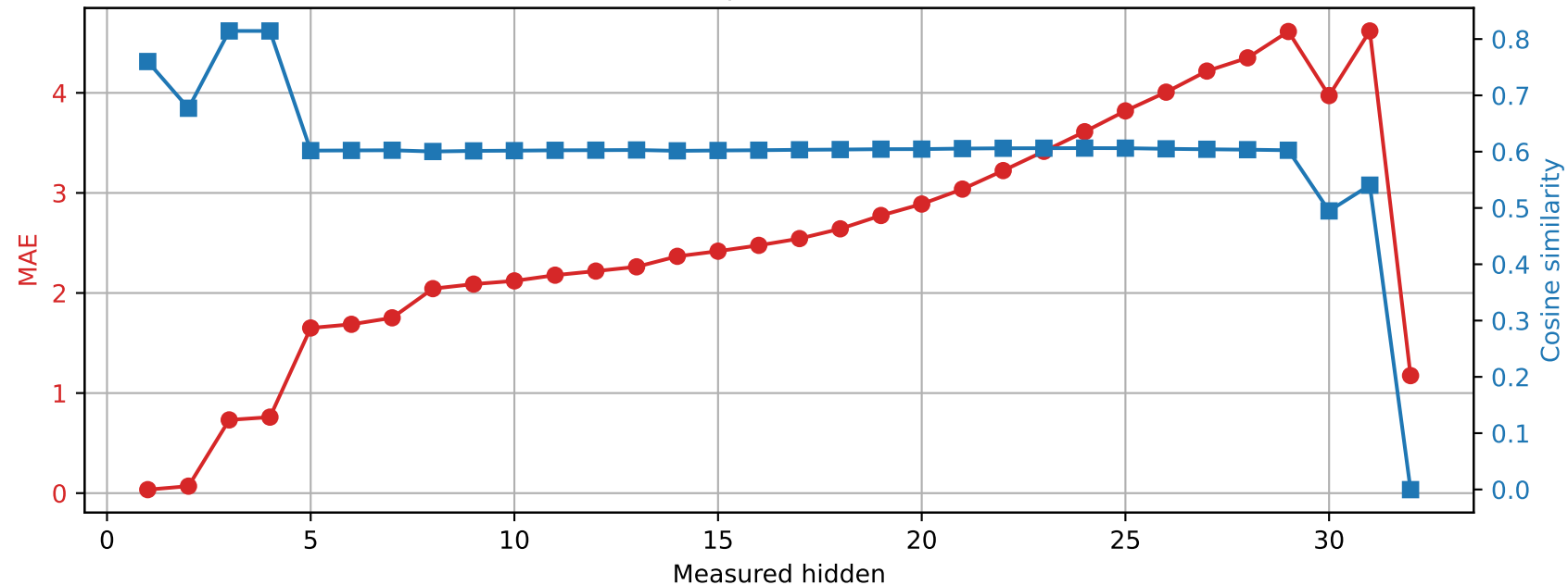
Phi-3-mini-4k-instruct | Prompt 0 Spared layer 29 | Unquantized vs hybrid
