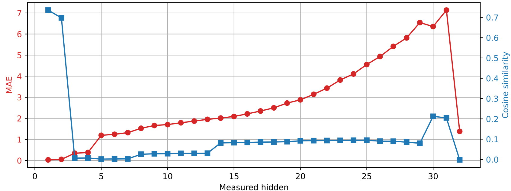
Phi-3-mini-4k-instruct | Prompt 2 Spared layer 8 | Unquantized vs hybrid
