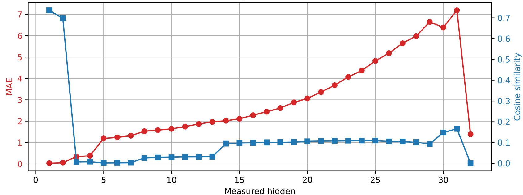
Phi-3-mini-4k-instruct | Prompt 2 Spared layer 31 | Unquantized vs hybrid
