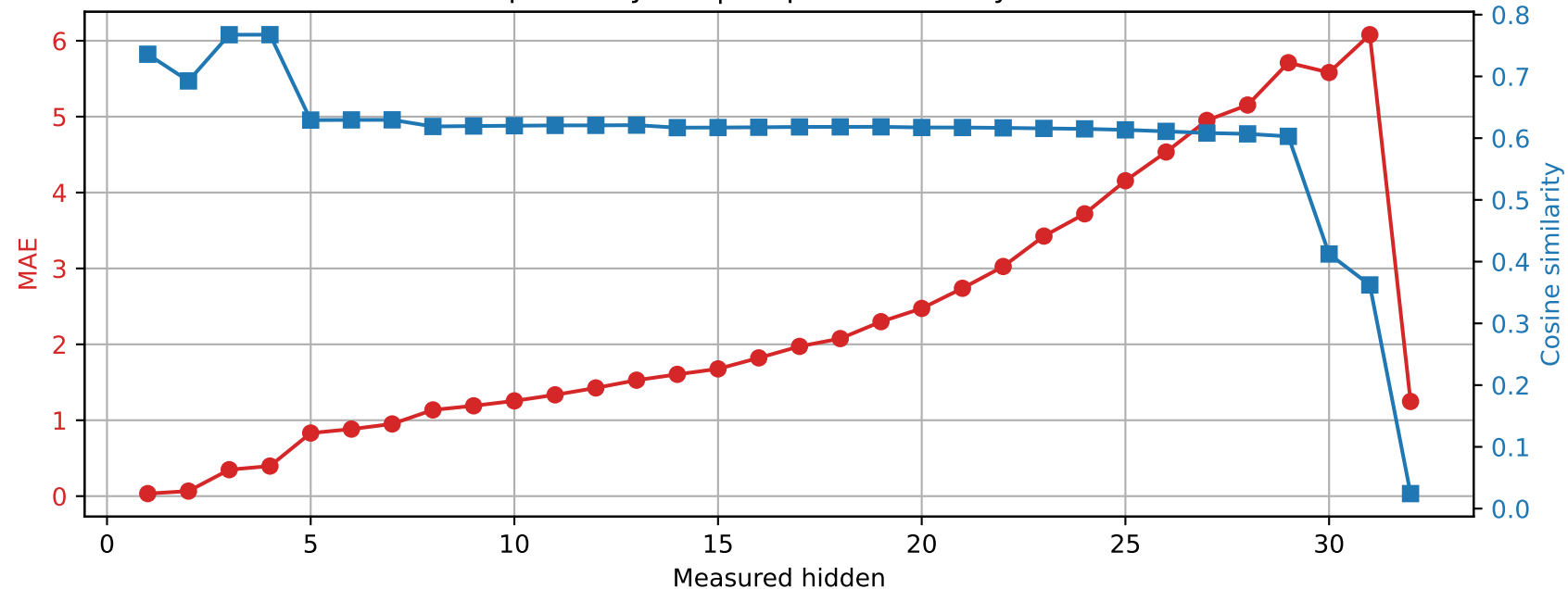
Phi-3-mini-4k-instruct | Prompt 3 Spared layer 3 | Unquantized vs hybrid
