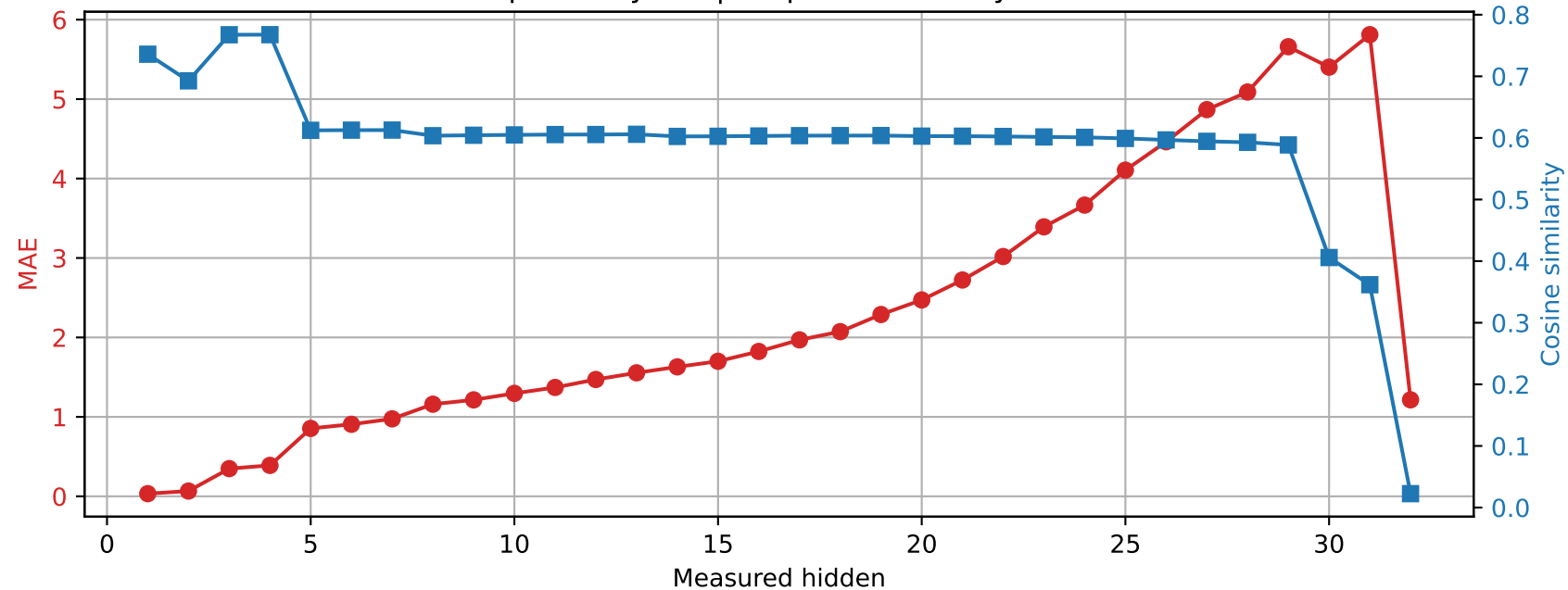
Phi-3-mini-4k-instruct | Prompt 3 Spared layer 9 | Unquantized vs hybrid
