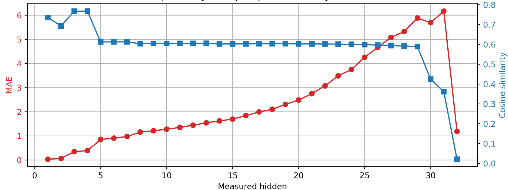
Phi-3-mini-4k-instruct | Prompt 3 Spared layer 28 | Unquantized vs hybrid
