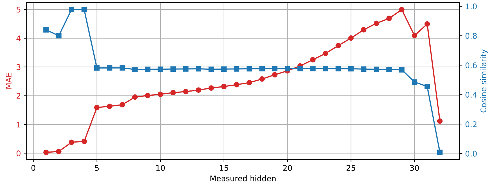
Phi-3-mini-4k-instruct | Prompt 4 Spared layer 1 | Unquantized vs hybrid
