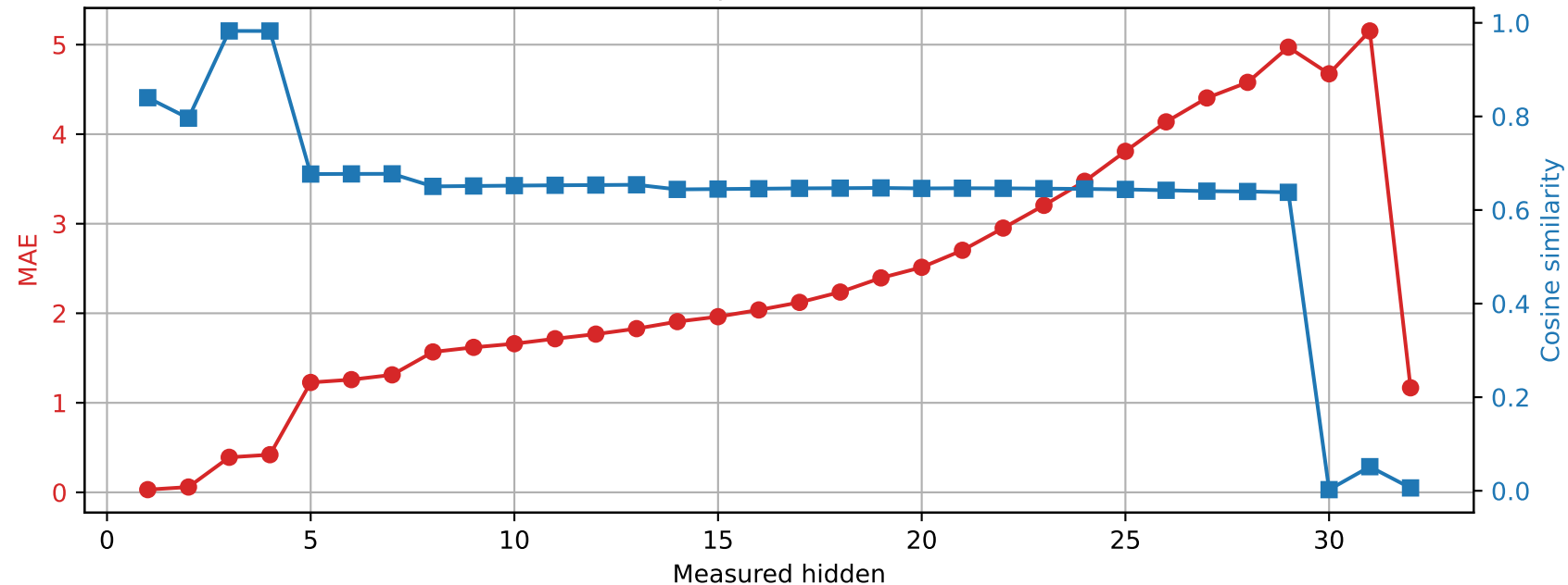
Phi-3-mini-4k-instruct | Prompt 4 Spared layer 4 | Unquantized vs hybrid
