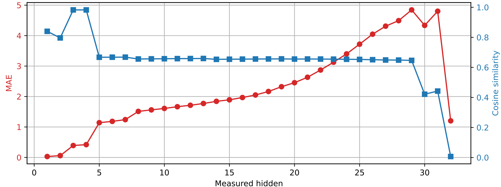
Phi-3-mini-4k-instruct | Prompt 4 Spared layer 7 | Unquantized vs hybrid
