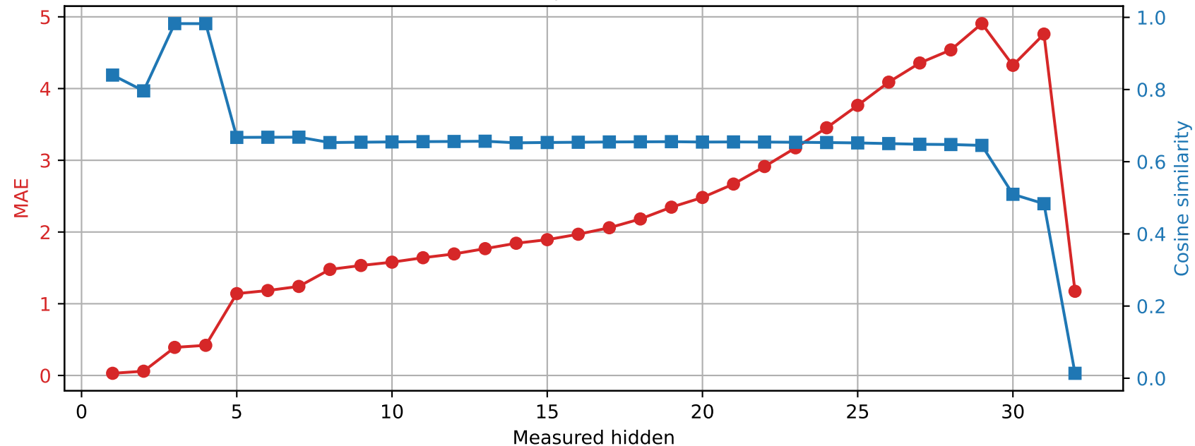
Phi-3-mini-4k-instruct | Prompt 4 Spared layer 12 | Unquantized vs hybrid
