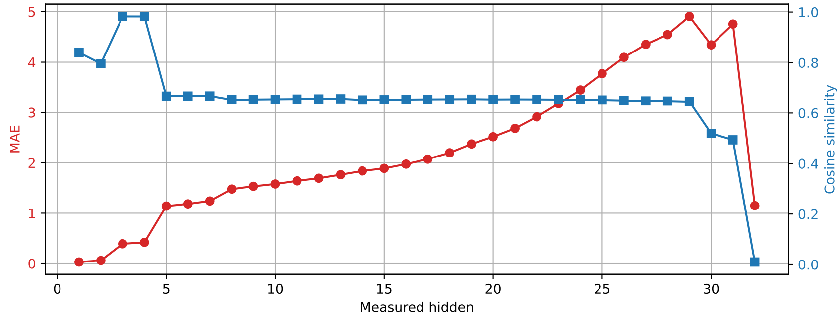
Phi-3-mini-4k-instruct | Prompt 4 Spared layer 20 | Unquantized vs hybrid
