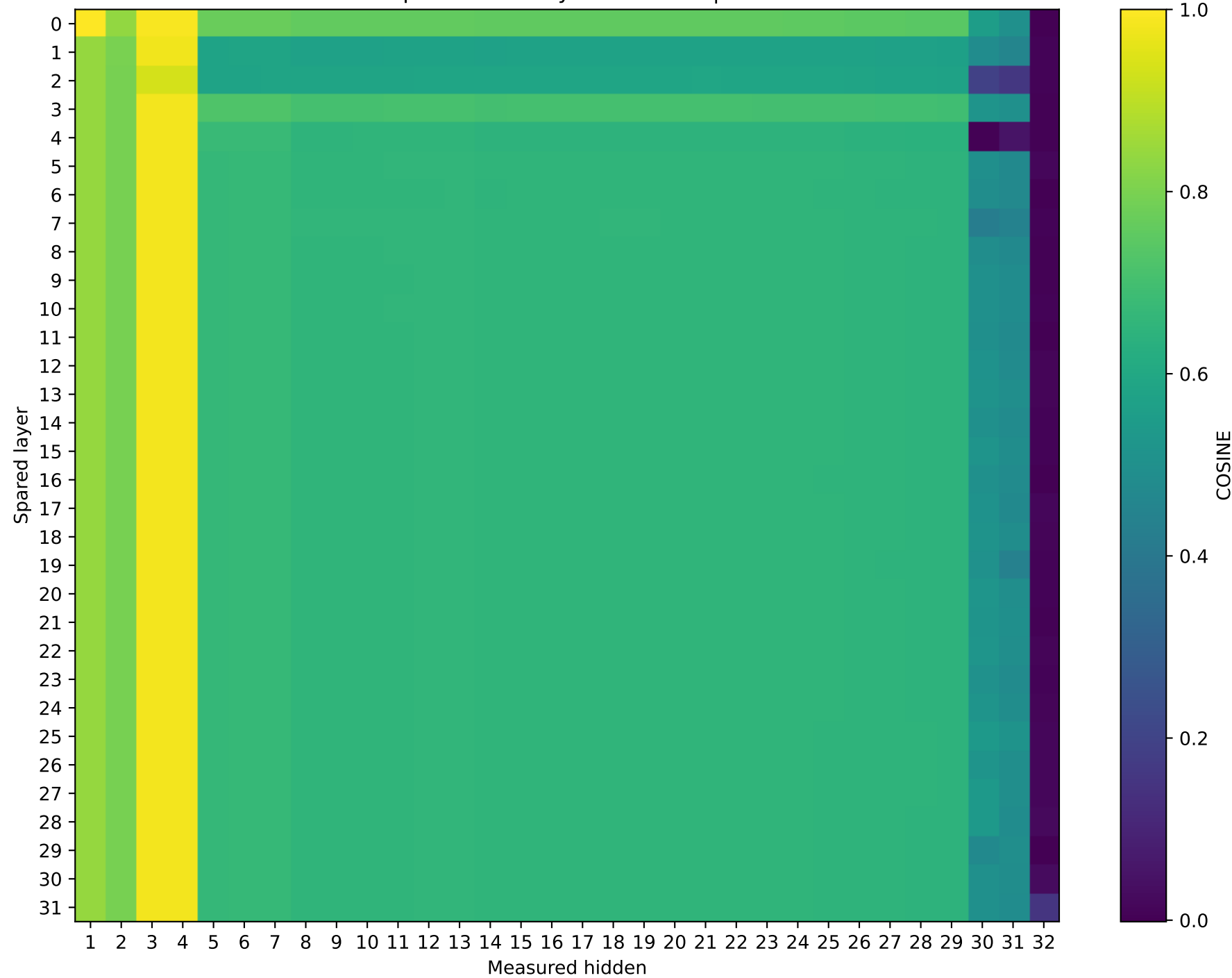
Phi-3-mini-4k-instruct | Prompt 4 Unquantized vs hybrid cos sim | int4
