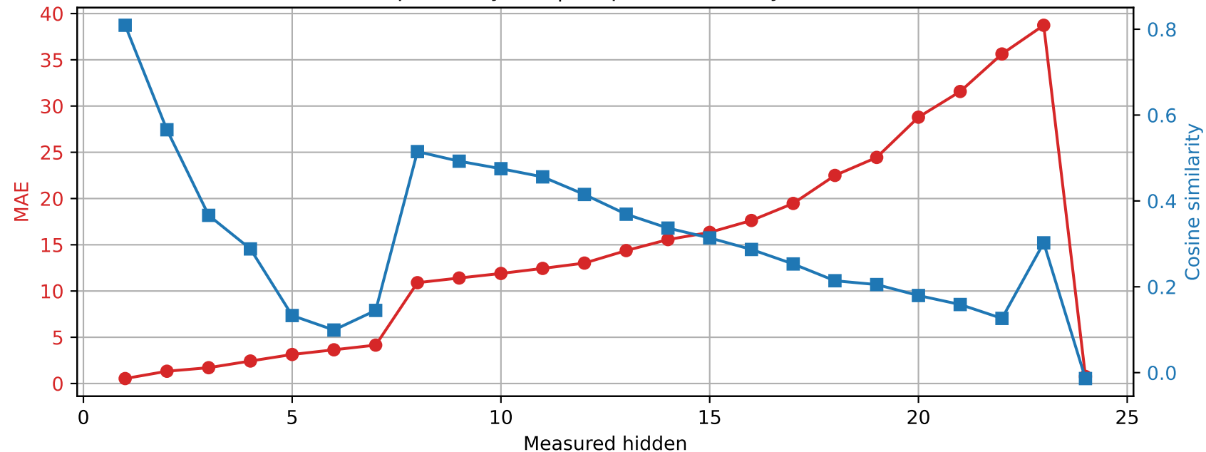
SmolLM2-1.7B-Instruct | Prompt 0 Spared layer 4 | Unquantized vs hybrid
