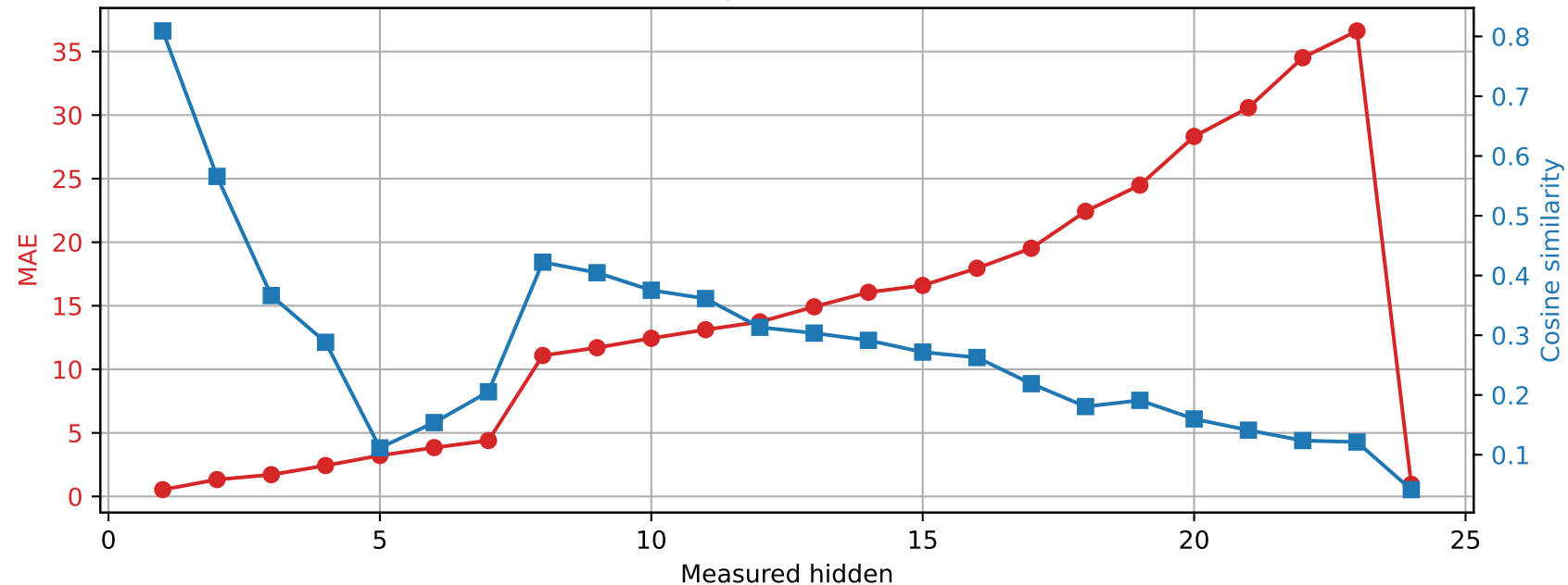
SmolLM2-1.7B-Instruct | Prompt 0 Spared layer 5 | Unquantized vs hybrid
