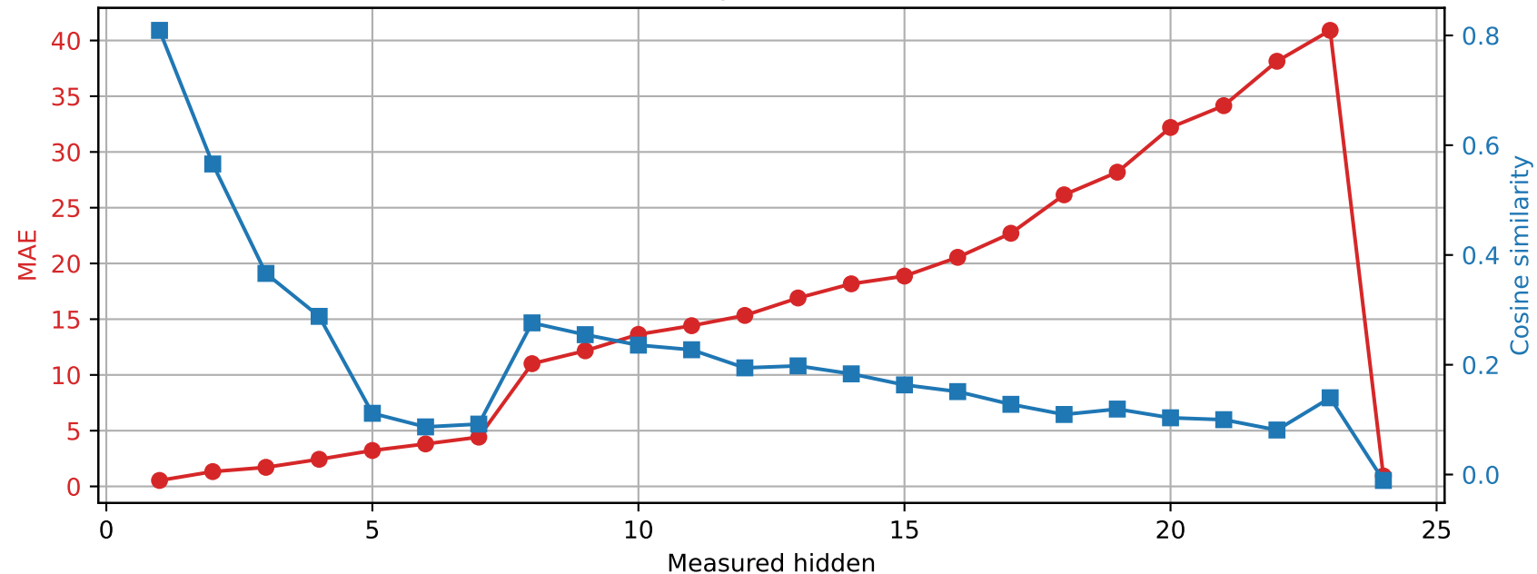
SmolLM2-1.7B-Instruct | Prompt 0 Spared layer 21 | Unquantized vs hybrid
