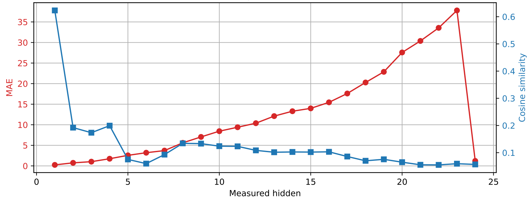
SmolLM2-1.7B-Instruct | Prompt 1 Spared layer 17 | Unquantized vs hybrid
