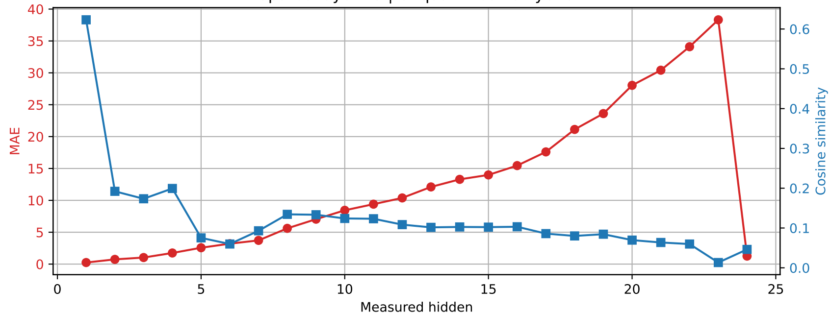
SmolLM2-1.7B-Instruct | Prompt 1 Spared layer 19 | Unquantized vs hybrid
