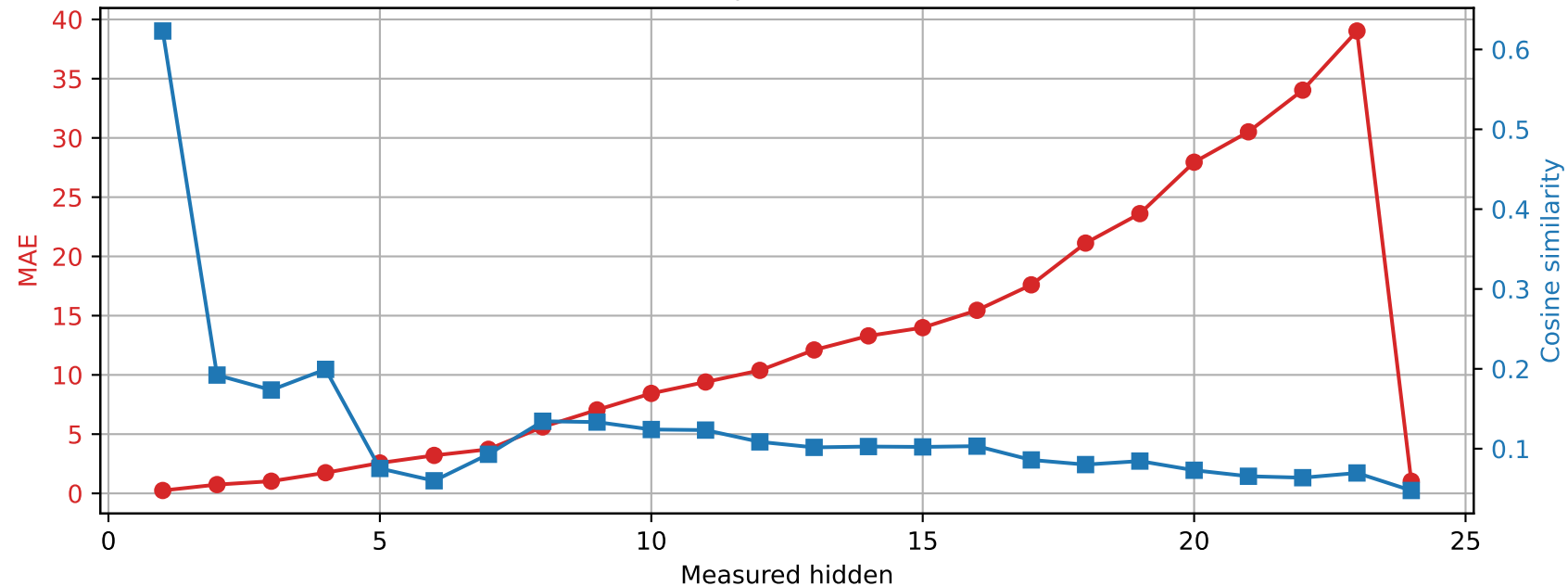
SmolLM2-1.7B-Instruct | Prompt 1 Spared layer 22 | Unquantized vs hybrid
