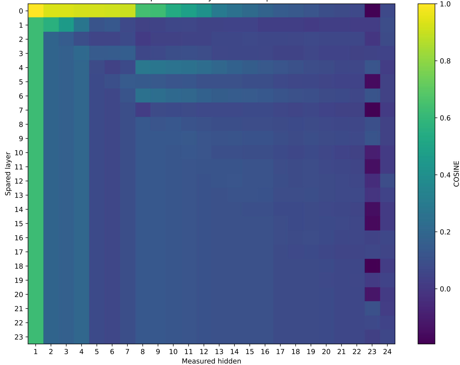
SmolLM2-1.7B-Instruct | Prompt 1 Unquantized vs hybrid cos sim | int4
