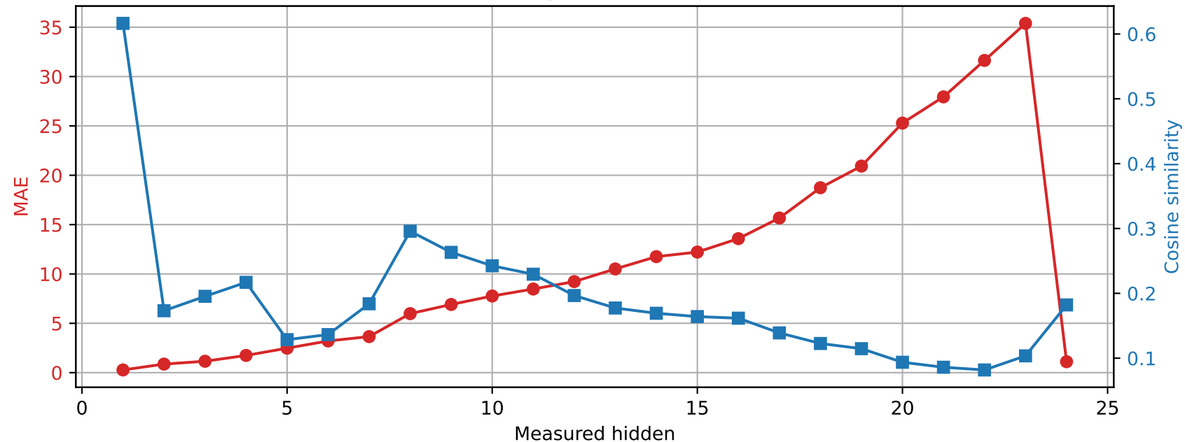
SmolLM2-1.7B-Instruct | Prompt 2 Spared layer 5 | Unquantized vs hybrid
