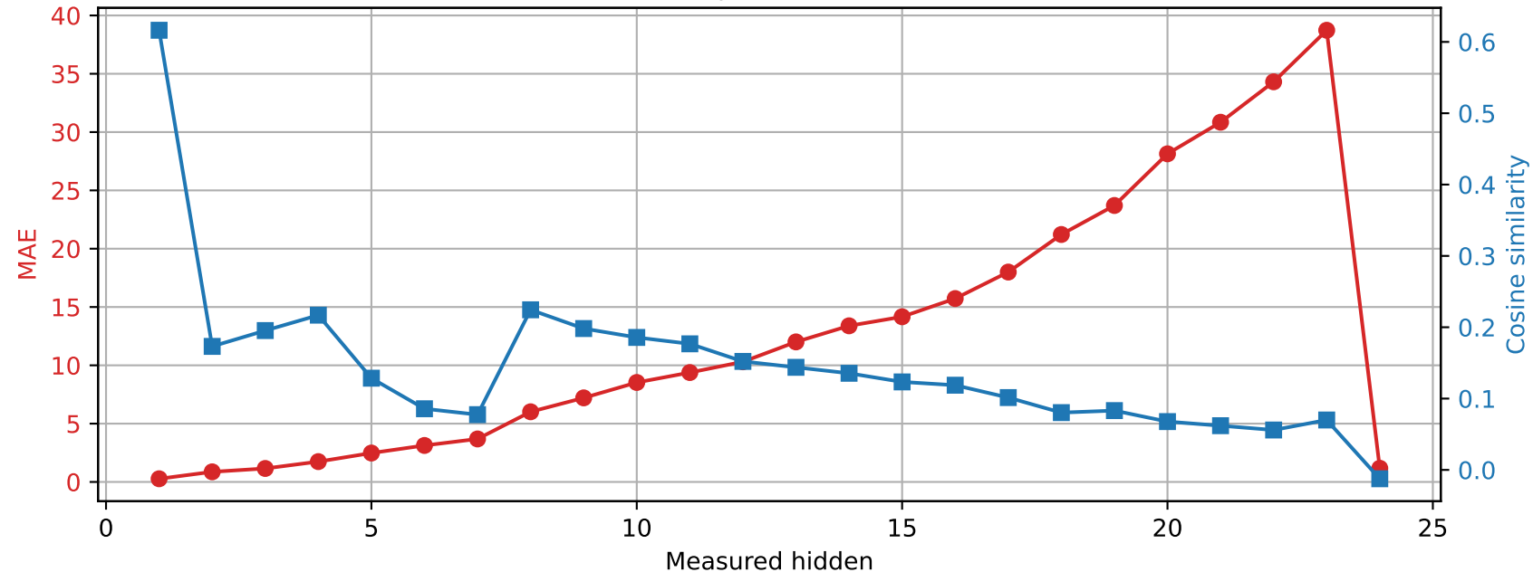
SmolLM2-1.7B-Instruct | Prompt 2 Spared layer 17 | Unquantized vs hybrid
