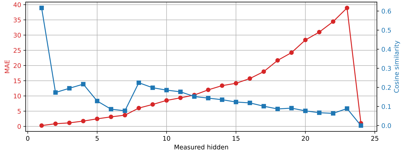
SmolLM2-1.7B-Instruct | Prompt 2 Spared layer 20 | Unquantized vs hybrid
