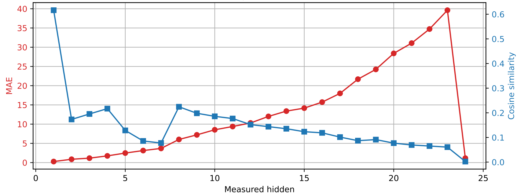
SmolLM2-1.7B-Instruct | Prompt 2 Spared layer 22 | Unquantized vs hybrid
