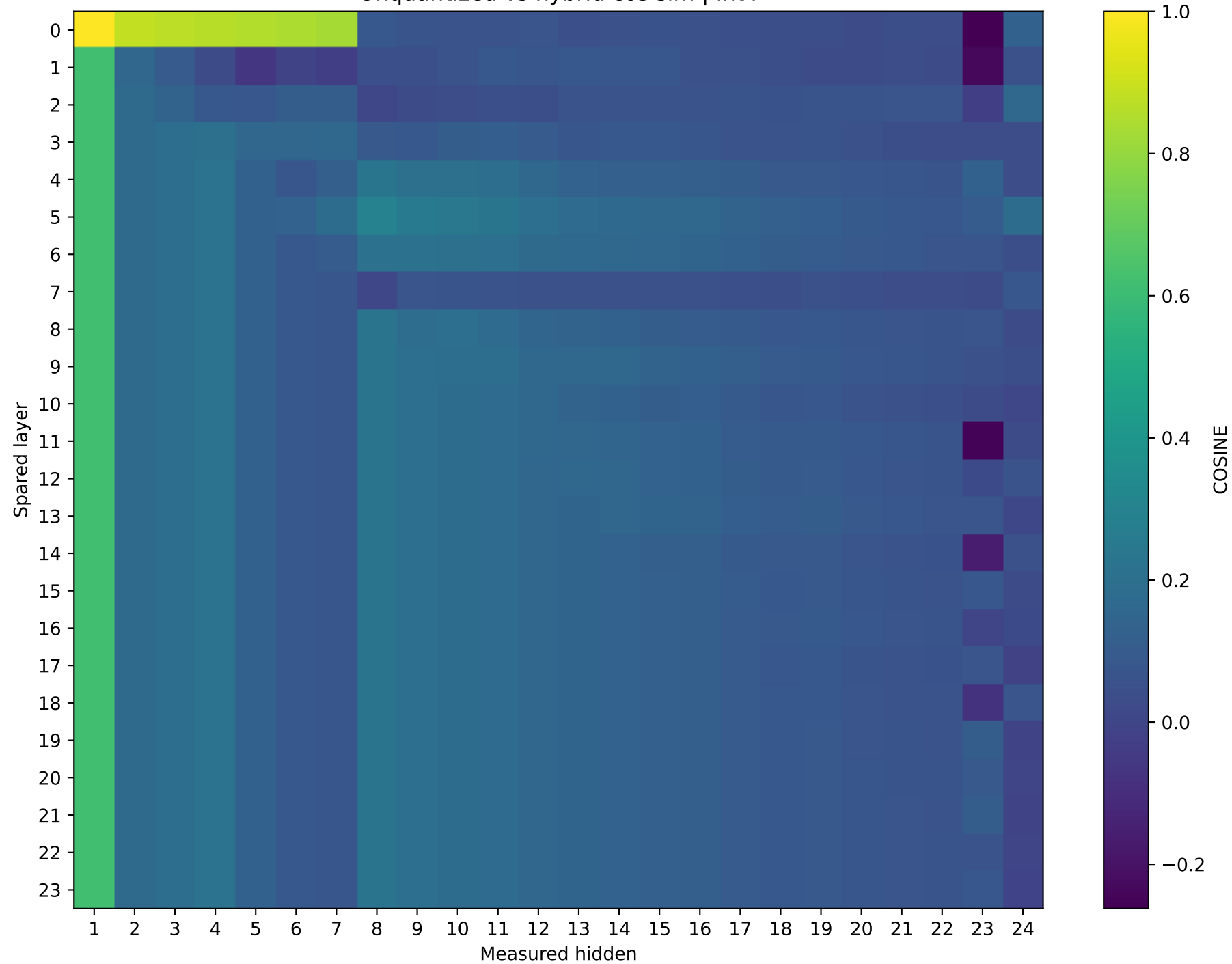
SmolLM2-1.7B-Instruct | Prompt 2 Unquantized vs hybrid cos sim | int4
