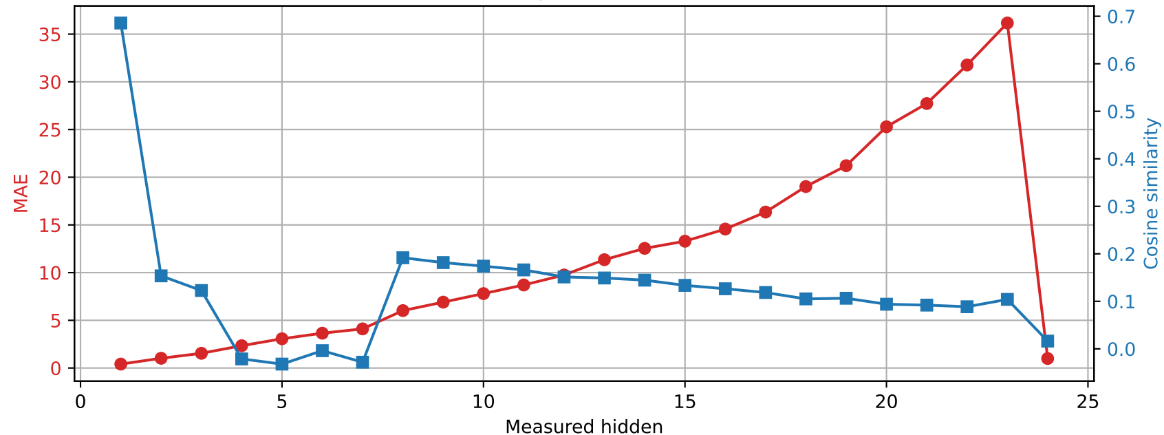
SmolLM2-1.7B-Instruct | Prompt 3 Spared layer 2 | Unquantized vs hybrid
