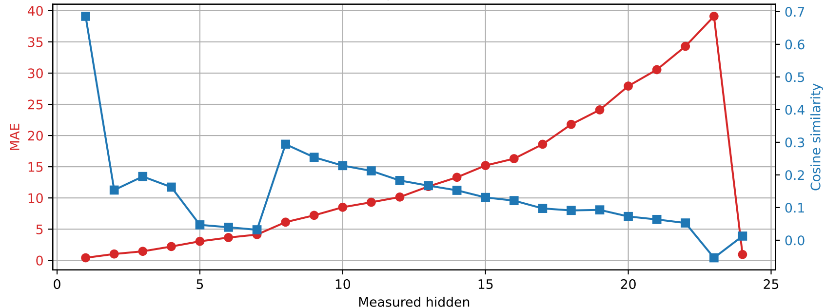
SmolLM2-1.7B-Instruct | Prompt 3 Spared layer 14 | Unquantized vs hybrid
