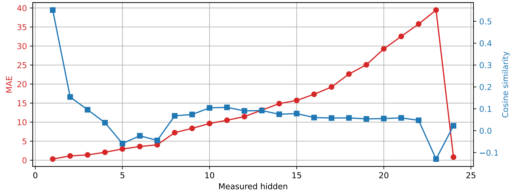
SmolLM2-1.7B-Instruct | Prompt 4 Spared layer 1 | Unquantized vs hybrid
