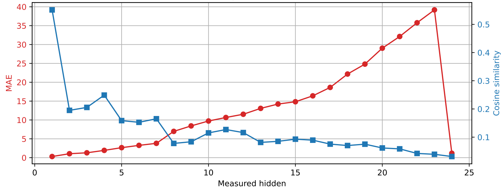
SmolLM2-1.7B-Instruct | Prompt 4 Spared layer 3 | Unquantized vs hybrid
