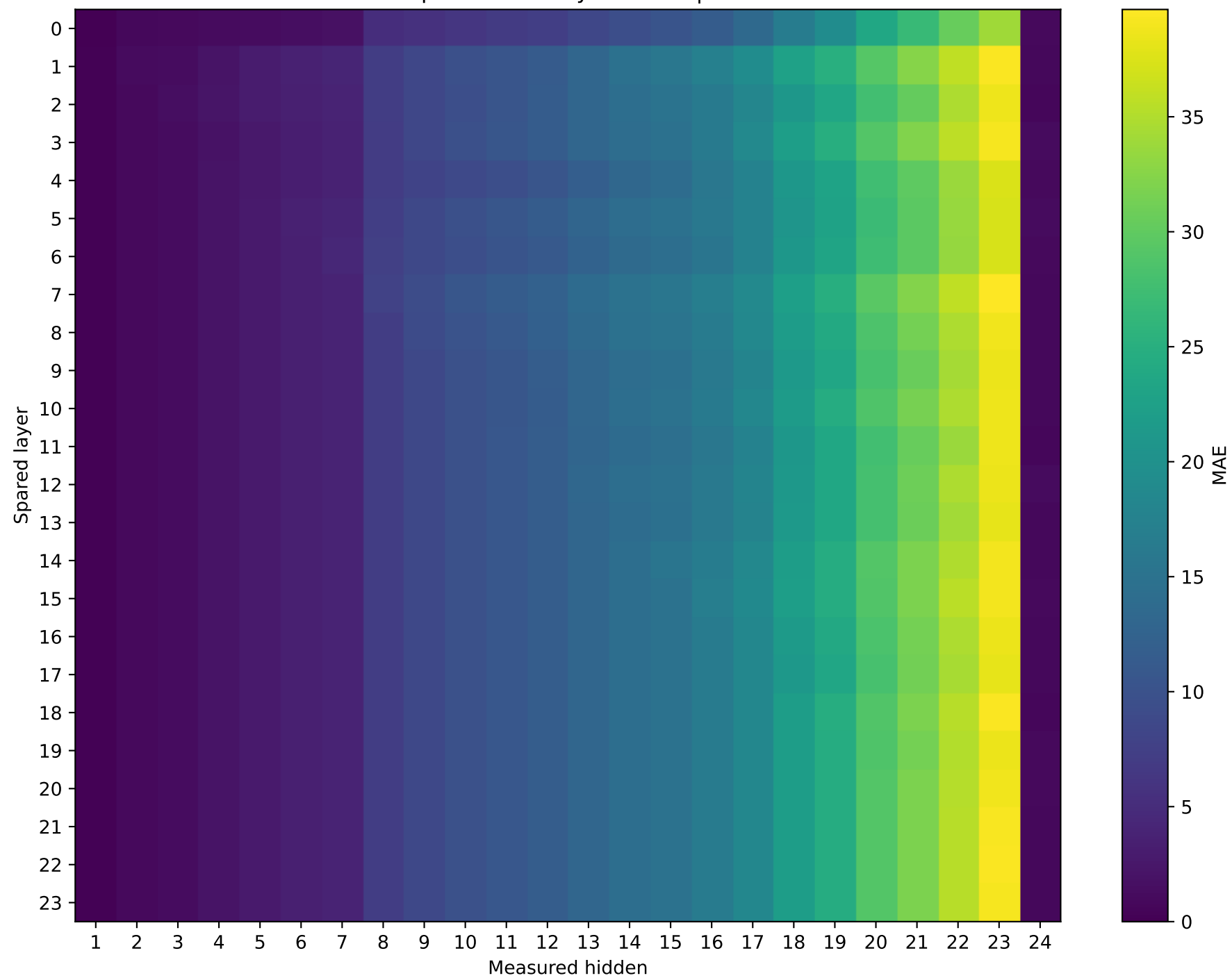
SmolLM2-1.7B-Instruct | Prompt 4 Unquantized vs hybrid MAE | int4
