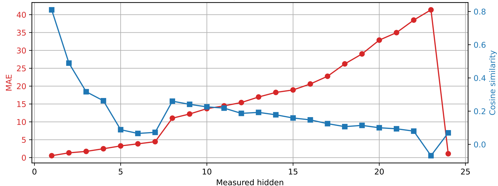
SmolLM2-1.7B-Instruct | Prompt 0 Spared layer 18 | Unquantized vs hybrid
