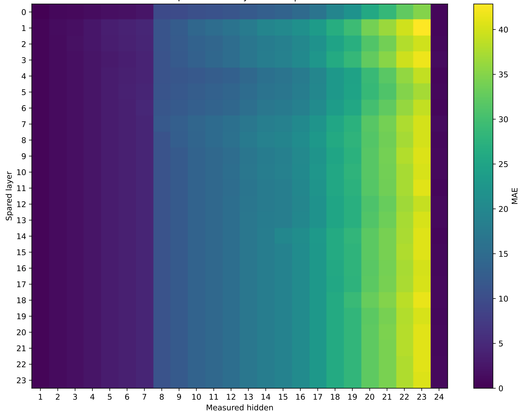
SmolLM2-1.7B-Instruct | Prompt 0 Unquantized vs hybrid MAE | int4
