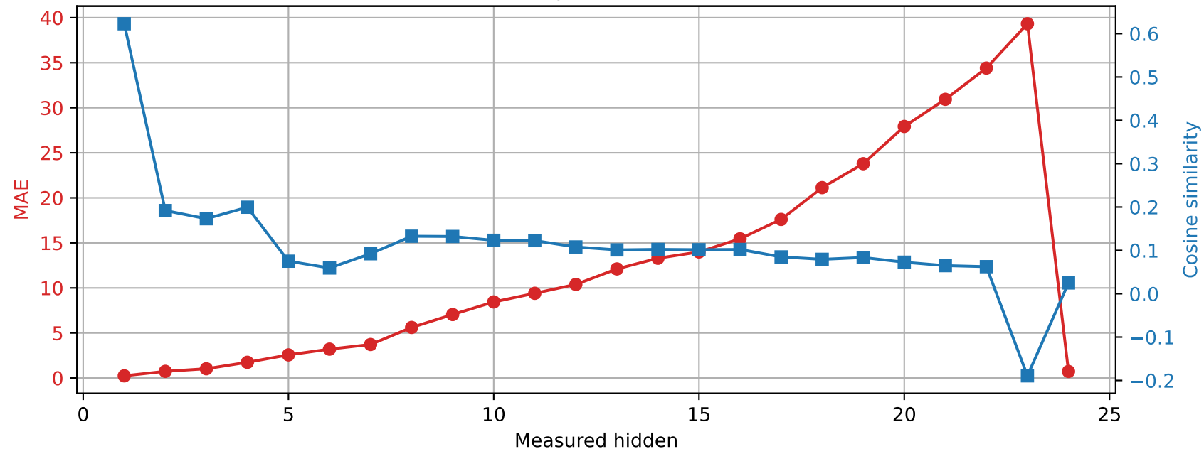
SmolLM2-1.7B-Instruct | Prompt 1 Spared layer 18 | Unquantized vs hybrid
