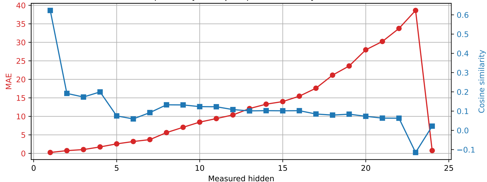
SmolLM2-1.7B-Instruct | Prompt 1 Spared layer 20 | Unquantized vs hybrid
