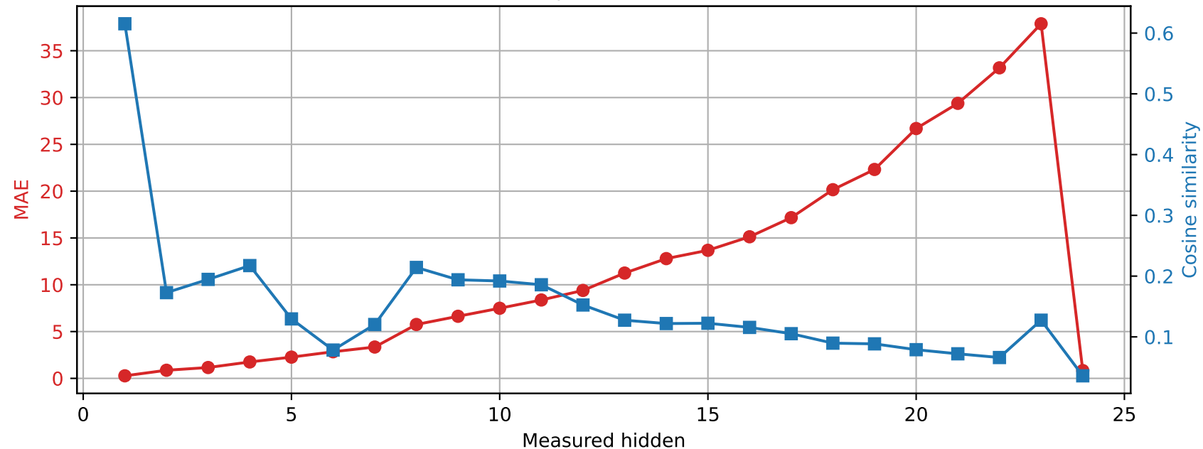
SmolLM2-1.7B-Instruct | Prompt 2 Spared layer 4 | Unquantized vs hybrid
