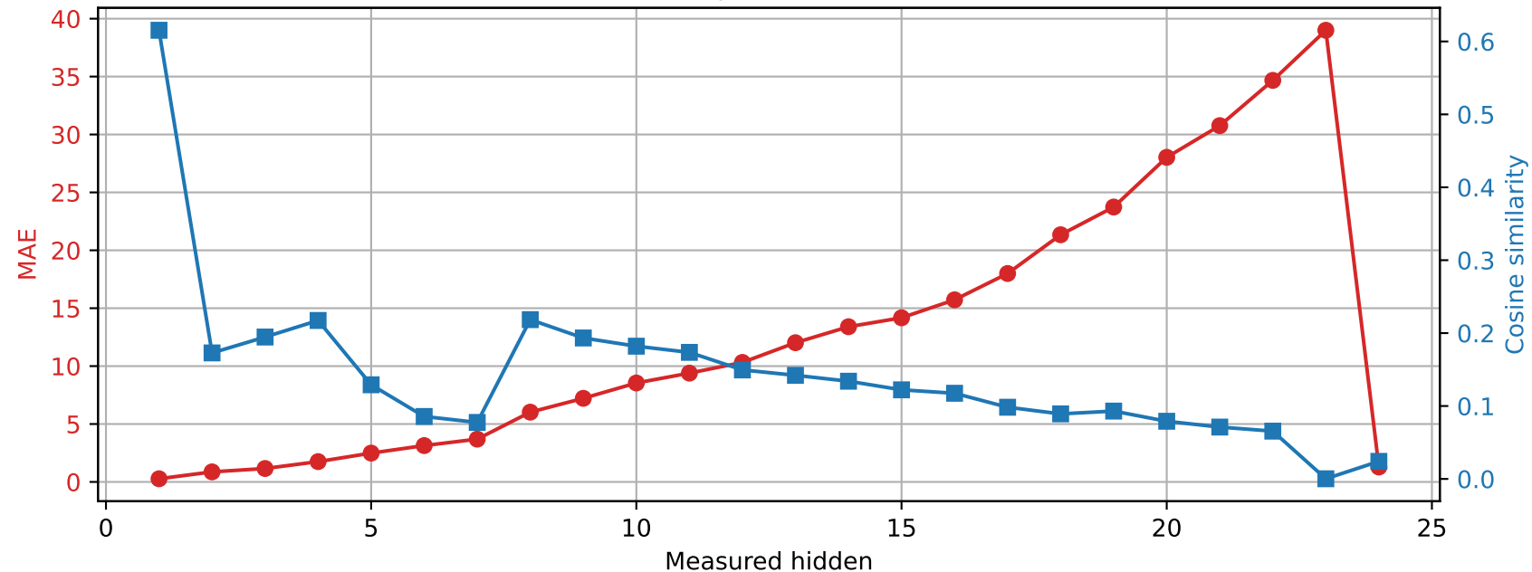
SmolLM2-1.7B-Instruct | Prompt 2 Spared layer 16 | Unquantized vs hybrid
